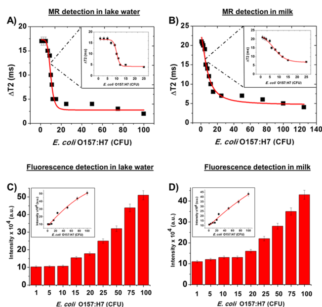
Figure 2. Magnetic relaxation \Delta T_2 data were collected in more complex media, including (A) lake water and (B) whole milk. Similar to the previous assays, it was noted that detection of bacterial contaminants was more sensitive in the range of 1–20 CFU (insets). Corresponding fluorescence data were collected for both the (C) lake water and (D) milk samples (insets: linearity plots) and showed higher sensitivity with higher CFU counts. Once again, these assays demonstrate the dual detection capabilities of our nanosensors and validate their accuracy in complex media.
